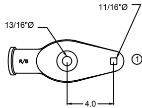
END FITTING VIEW - "AA" OR "AASC"
