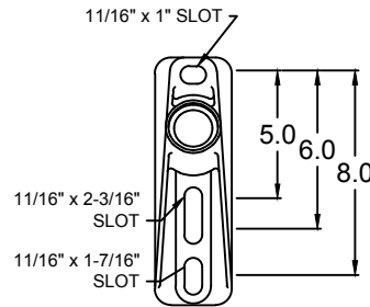
BASE VIEW >GPB5568MBC
