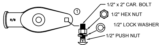
END FITTING VIEW - "AAB" OR "AABC"
