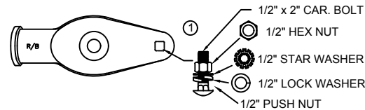
END FITTING VIEW - "AAW"
