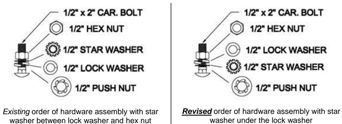
Figure 1 – Order of hardware assembly on fiberglass brackets with a star washer option
